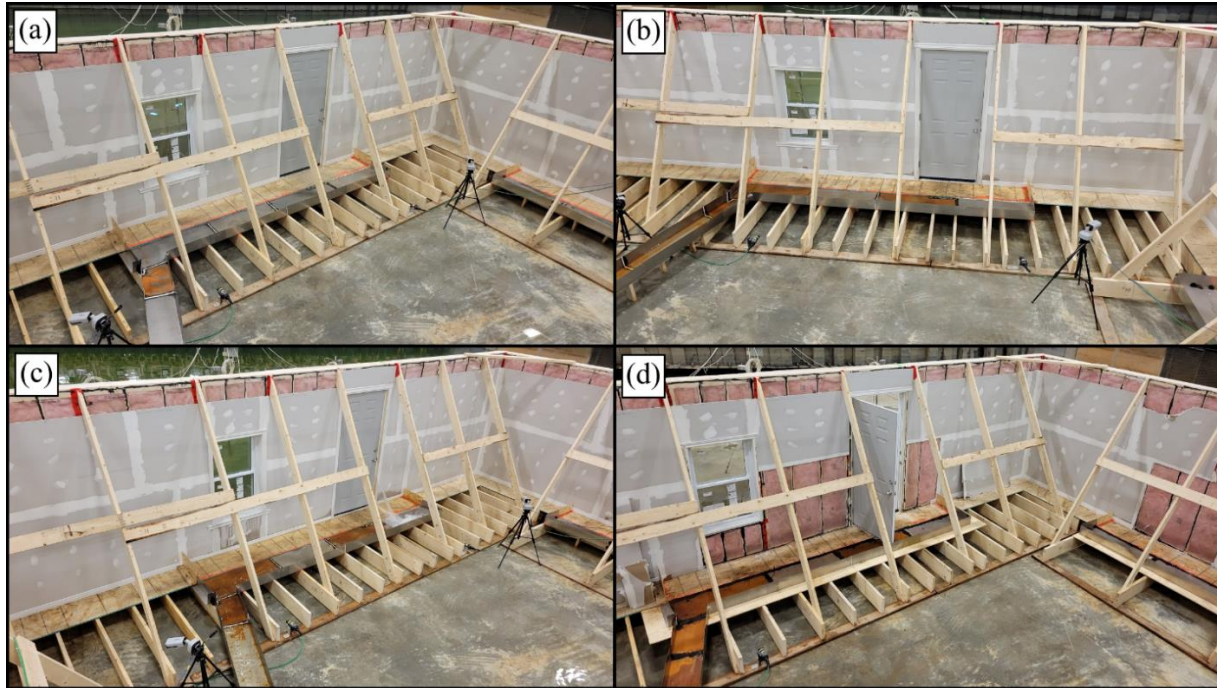
Figure 36. Evolution of water damage to Phase 1 superstructure. (a) Before the start of testing; (b) after the TSA; (c) during TSD; (d) during the deconstruction process. Note – the drywall was removed as part of the deconstruction, not by the flood waters.
