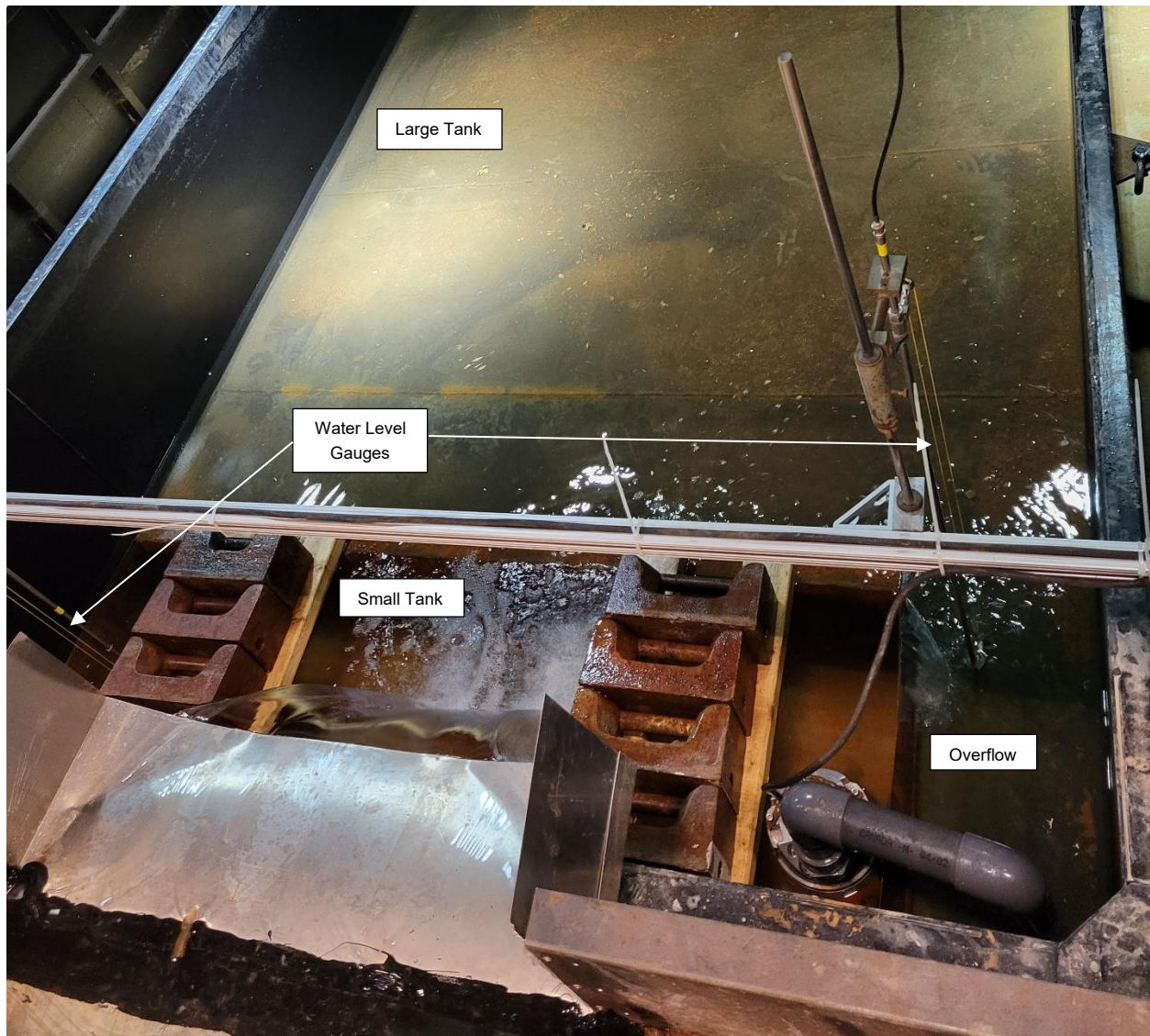
Figure 17. Leakage rate measuring tanks within the dry pit for Phase 1.
