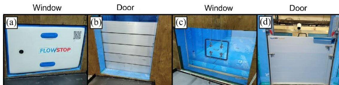
Figure 23. Opening barriers deployed in the IT in Phase 2: (a) Flow Stop full-sized cushion; (b) Stormmeister Rapid Assembly Log type Barrier; (c) Aqualock Window Protector; and (d) Aqualock Quickwall.
