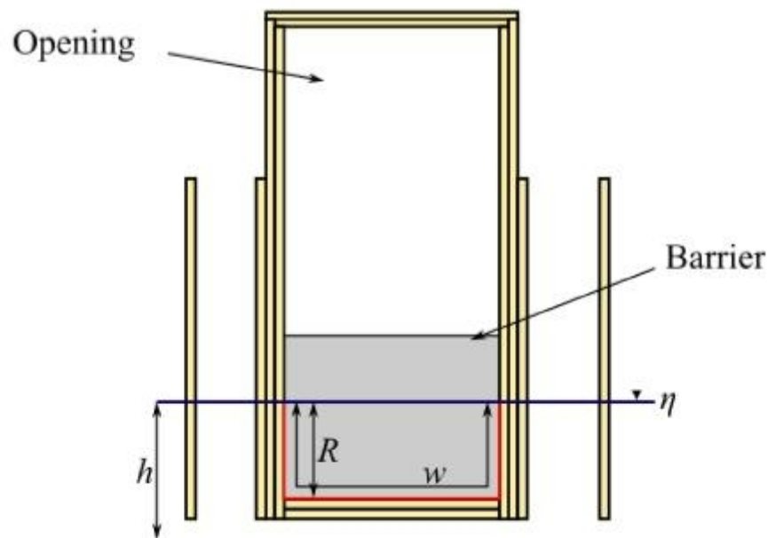
Figure 24. Important parameters for the analysis of leakage rate through the temporary barriers.
