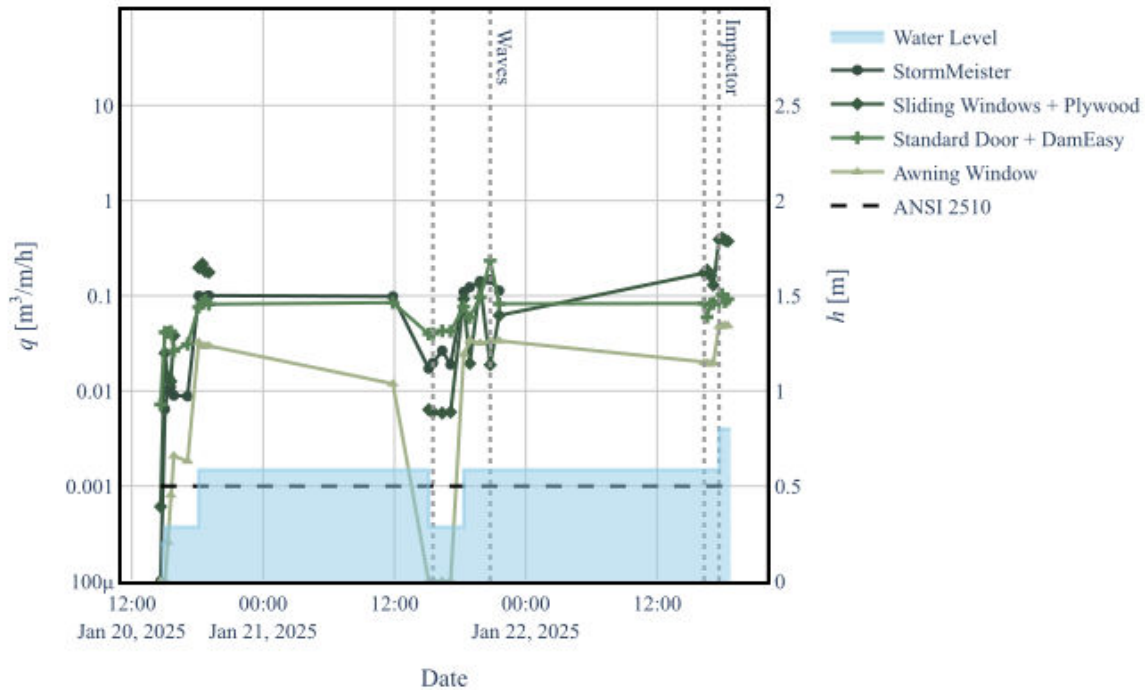
Figure 46. Leakage rate per opening width for the third test series in the MWB.
