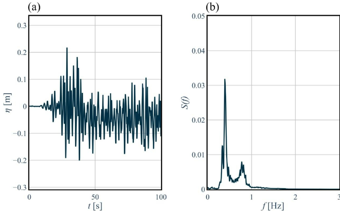
Figure 29. Frequency analysis of wave time series (WP01). (a) Time series of water surface elevation; (b) frequency analysis of water surface elevation.
