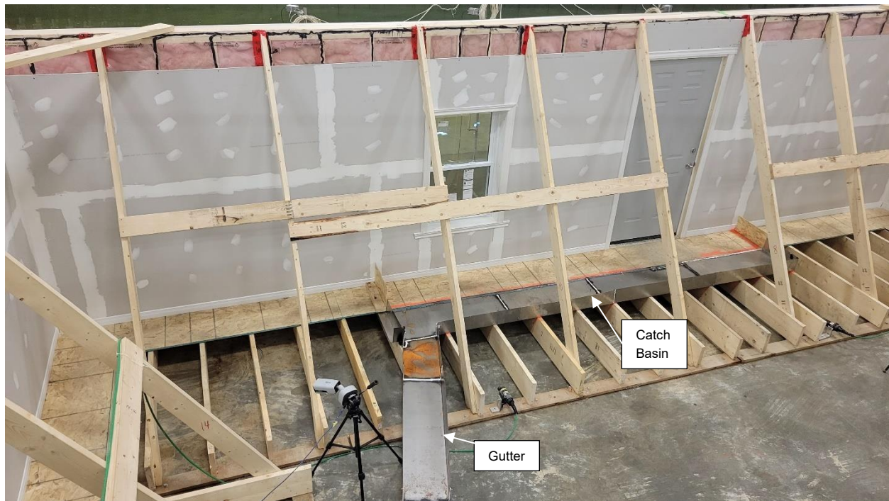
Figure 16. Catch basin system for measuring leakage rates from the door and window openings during Phase 1. A gutter leads from the catch basing towards the dry pit.
