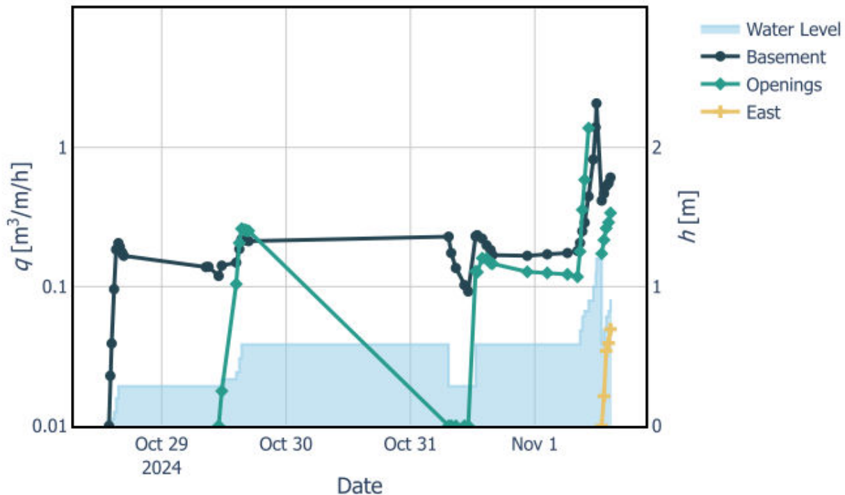
Figure 35. Leakage rate per unit width through the Phase 1 superstructure. The water levels are given in absolute coordinate (referenced to the floor of the raised platform). Time is given in Eastern Standard Time (EST).
