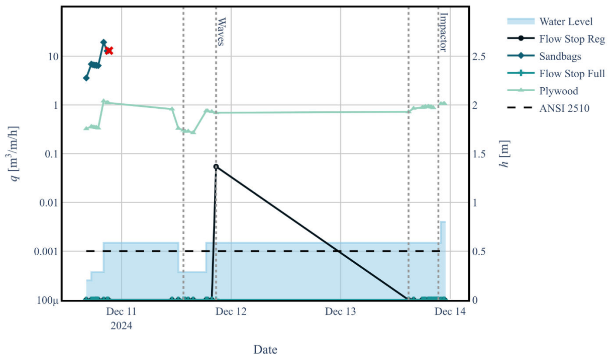
Figure 43. Leakage rate per width of the opening for second test series in the MWB.
