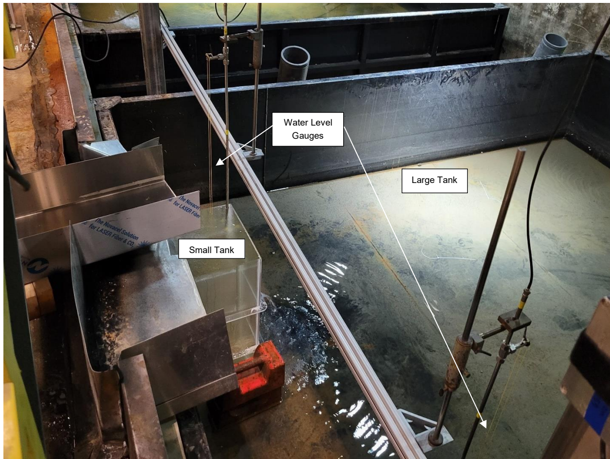
Figure 19. Leakage rate measuring tanks within the dry pit for Phase 2.
