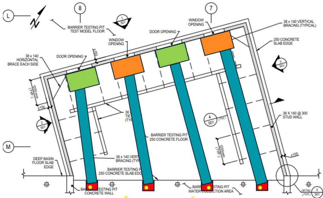
Figure 18. Catch basin system for measuring leakage rates for Phase 2. In green we have the catch basins for the two door openings, in orange we have the catch basin for the two window openings.
