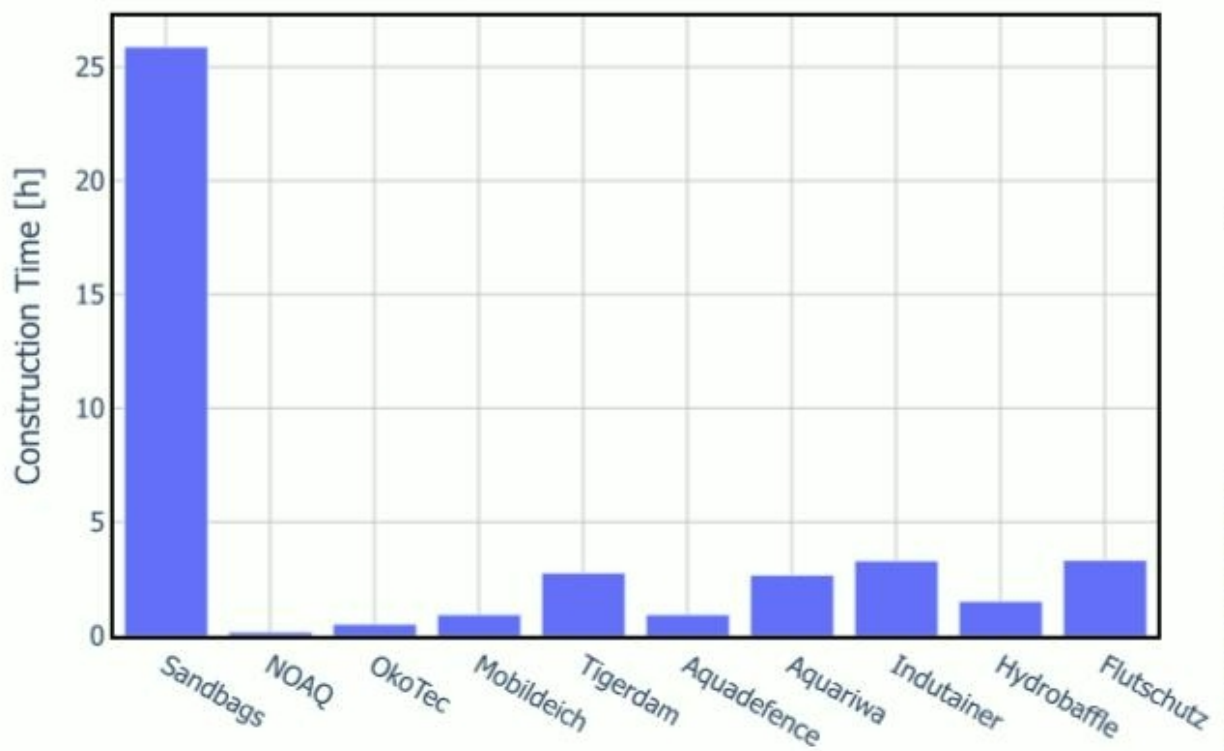
Figure 6. Construction time for 15 m of various perimeter barrier technologies (adapted from Massolle et al. (2018)).
