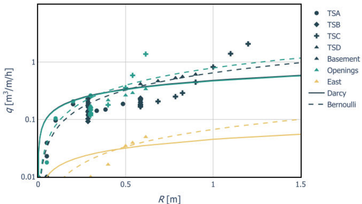
Figure 39. Leakage rate per unit meter versus the relative freeboard through the Phase 1 superstructure. The water level is referenced to the height of the opening: 0.285 m for the opening and east and 0 m for the basement. Lines are the fitted parameters from Table 8.
