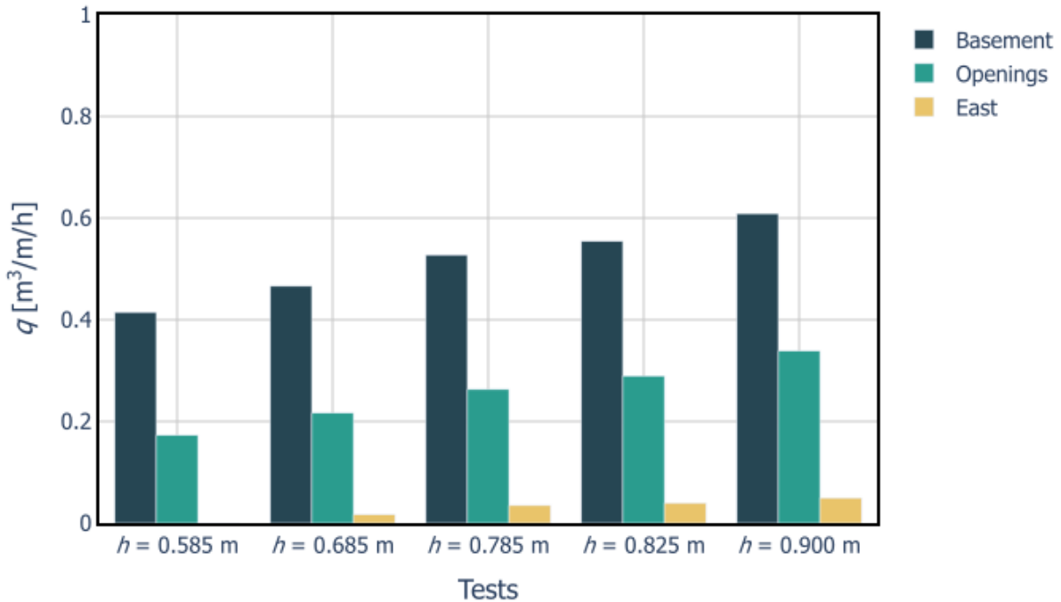
Figure 40. Influence of water depth on leakage rate through Phase 1 structure.
