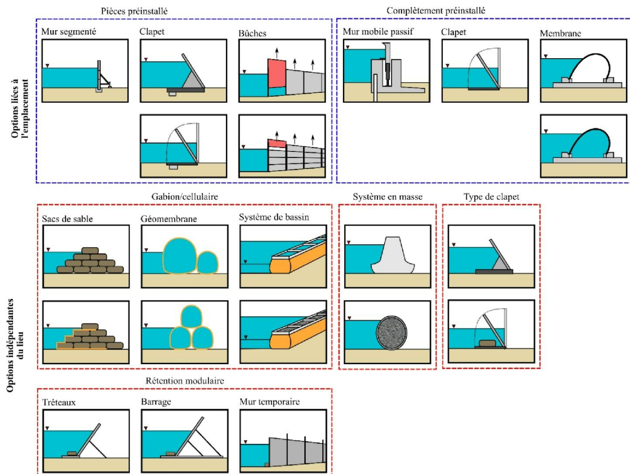
Figure 3. Classification system of perimeter barriers adapted from Massolle et al. (2018) and Biggar & Masala (1998)
