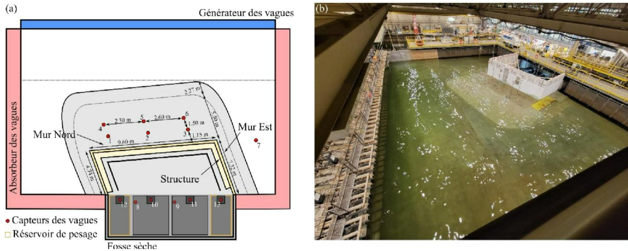
Figure 8. Plan view of the experimental facilities at the NRC. (a) Conceptual sketch of superstructure and instrument positions; (b) photo of Phase 1 testing of waves.
