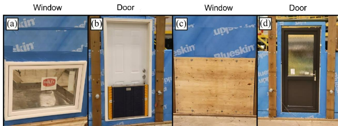
Figure 22. Opening Barriers deployed in the MWB during Phase 2 – third set of tests: (a) Awning window; (b) Standard Door with DamEasy; (c) Sliding Window with plywood; and (d) Stormmeister Flood Resistant Door.
