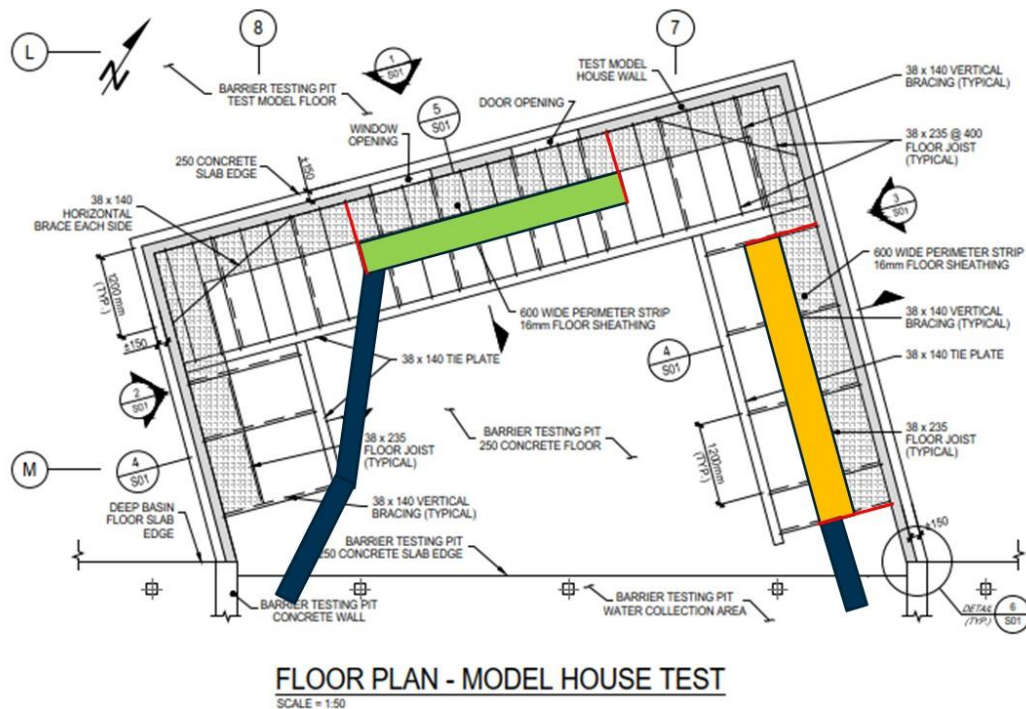
Figure 15. Catch basin system for measuring leakage rates for Phase 1. In green we have the catch basin for the door and window openings; In yellow we have the catch basin for the east wall.
