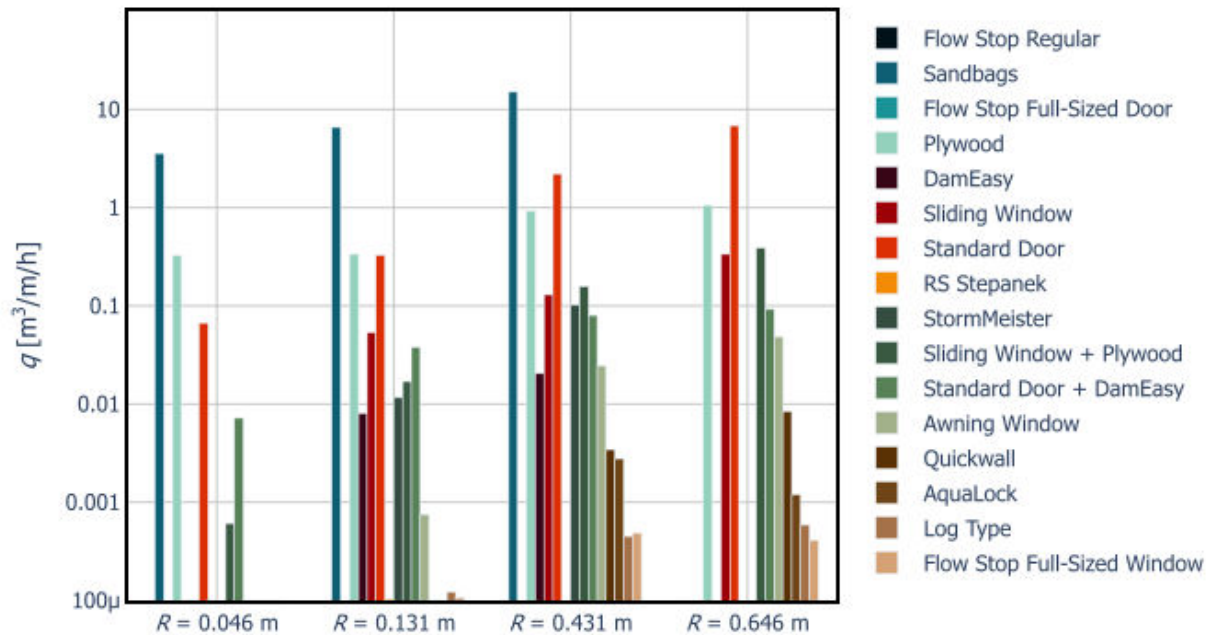
Figure 51. Average leakage rate per unit width as a function of freeboard for each of the barriers tested in Phase 2. The figure combines the tests from the MWB and IT.
