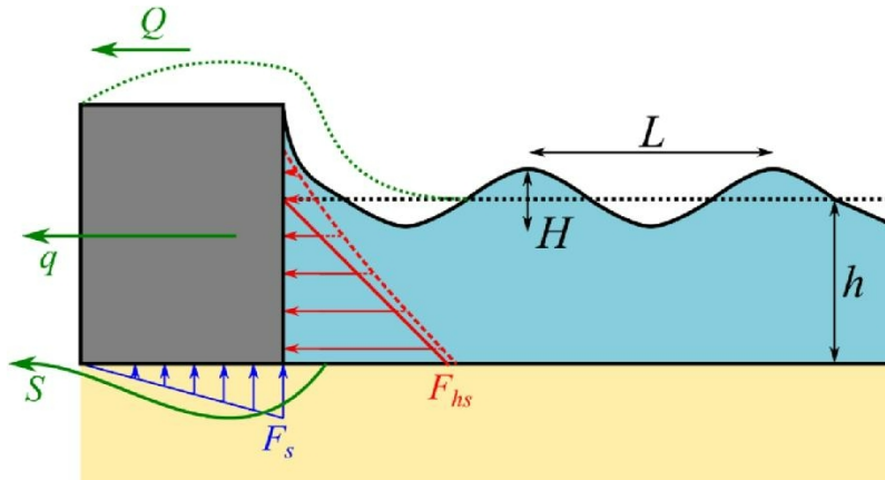
Figure 4. Forces on a flood barrier. H is the wave height, h is the water depth, L is the wavelength, F_{hs} is the hydrostatic force, F_s is the lift force, Q is the overtopping rate, q is the leakage rate, and S is the seepage rate.
