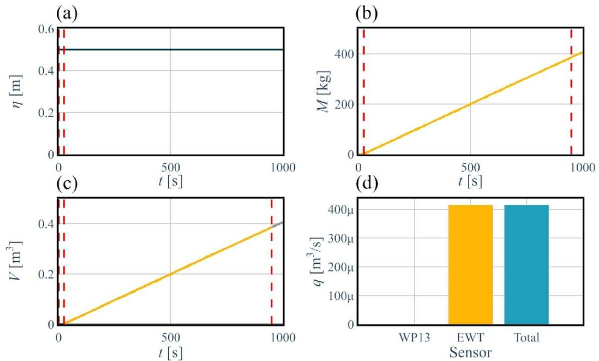
Figure 27. Leakage rates calculation taken from Phase 2: TSE – plywood board over east window opening. (a) water level measurements (WP13) in small tank; (b) weight tank measurements (EWT); (c) combined volume measurements from the two measurement methods; and (d) leakage rates measurements from two methods.
