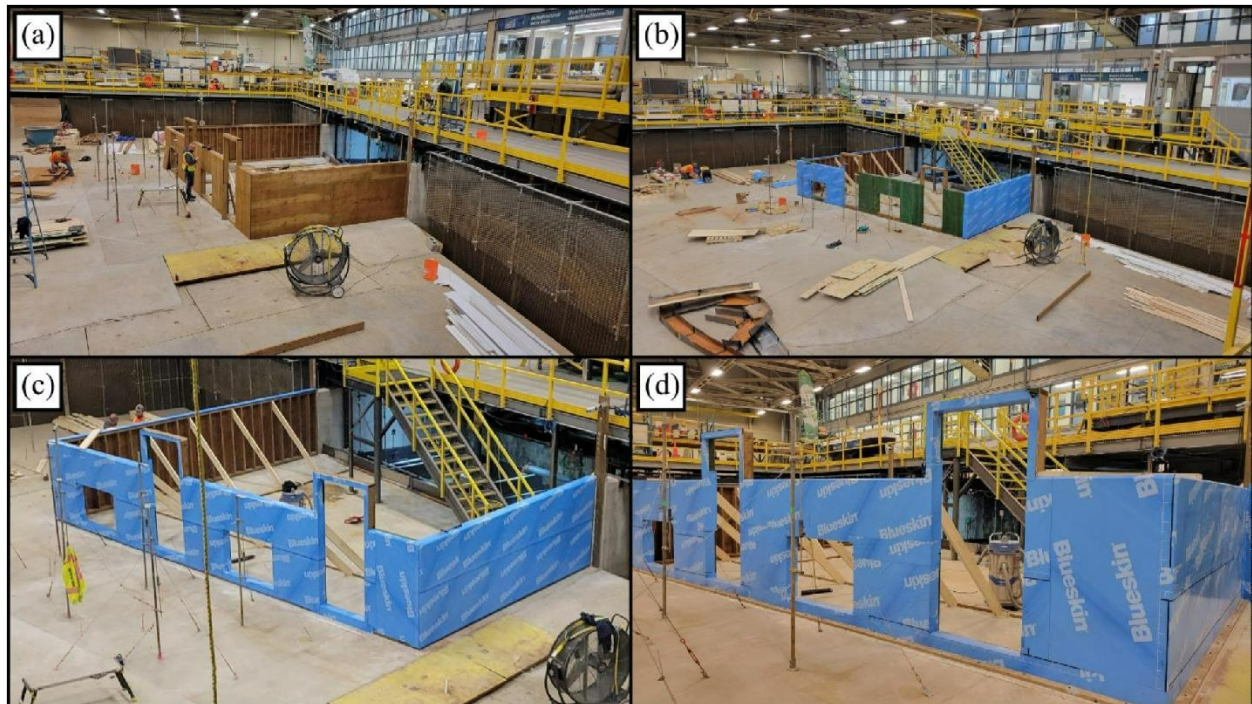
Figure 12. Construction of the Phase 2 impermeable structure. (a) Wood framing of structure; (b) placement of the waterproofing membrane; (c) completed waterproofing membrane; and (d) door and window openings.
