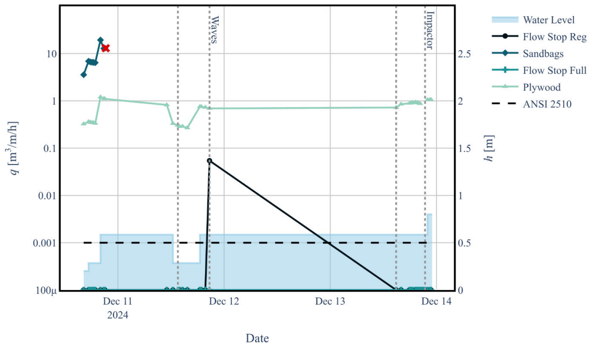
Figure 42. Leakage rate per width of the opening for first run through the experimental protocol in the MWB.
