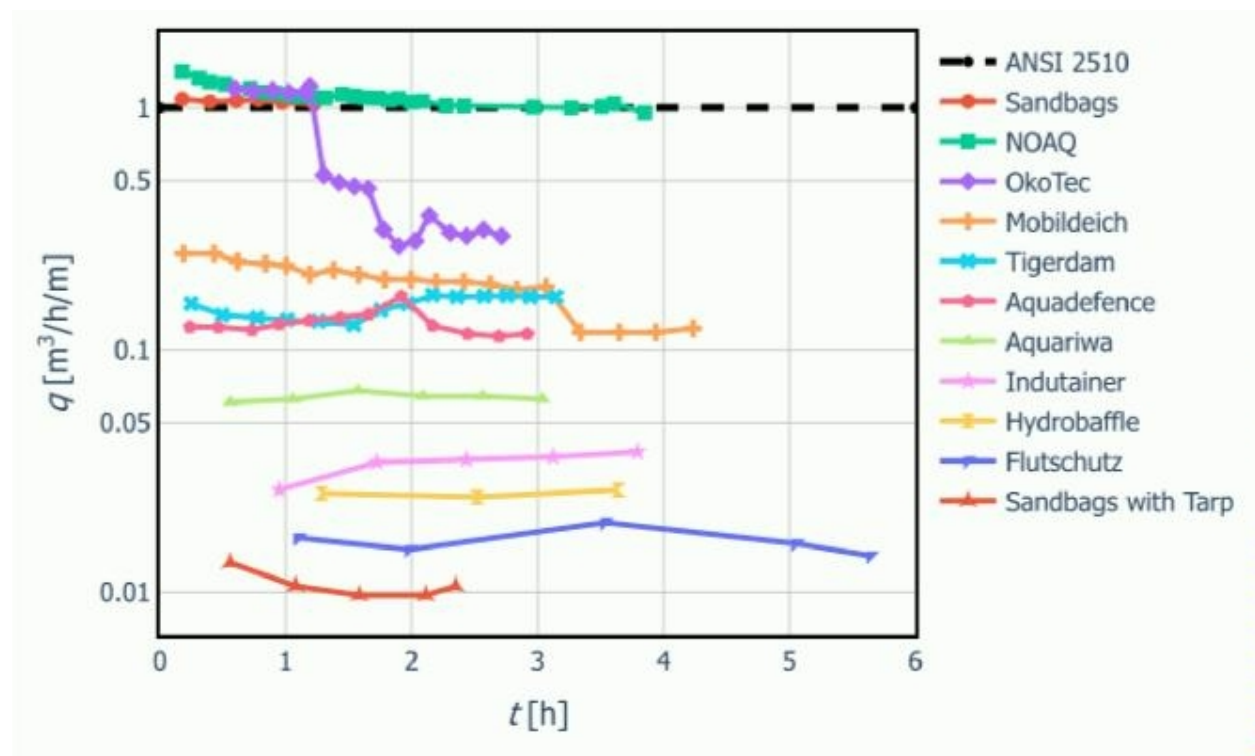
Figure 7. Combined (leakage, seepage, and overtopping) rate for various perimeter barriers (adapted from Massolle et al. (2018)) under a hydrostatic load with 0.60 m water depth.
