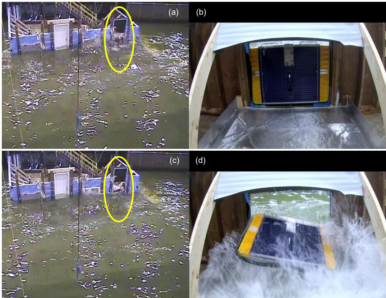
Figure 45. Failure of the DamEasy barrier under wave action. (a) shows the wave crashing against the structure, (b) shows the barrier as the wave crashes, (c) and (d) show the barrier at the moment of failure.
