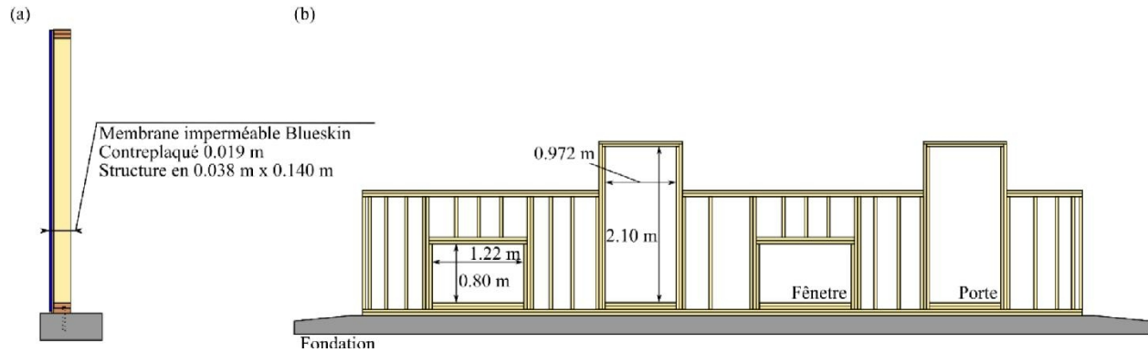
Figure 11. Conceptual drawing of Phase 2 structure. (a) Cross-section of the superstructure; (b) front view of the superstructure frame.
