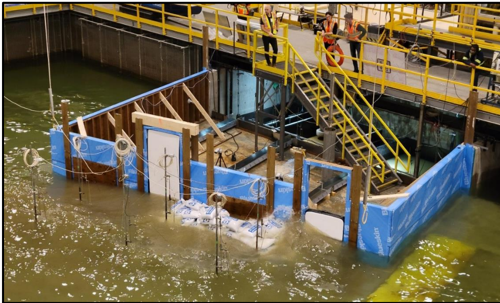
Figure 1. Phase 2 wave tests of four opening flood barriers in the National Research Council's (NRC) Multidirectional Wave Basin (MWB). From left to right: plywood, Flow Stop full sized cushion (Mono), sandbags and Flow Stop regular cushion (Bi).
