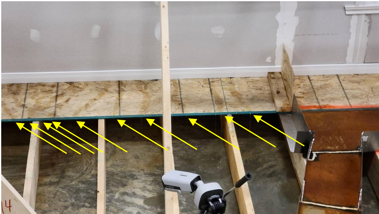
Figure 34. Leakage through the wall cavity in Phase 1. Water trickling off the subfloor identified with yellow arrows.
