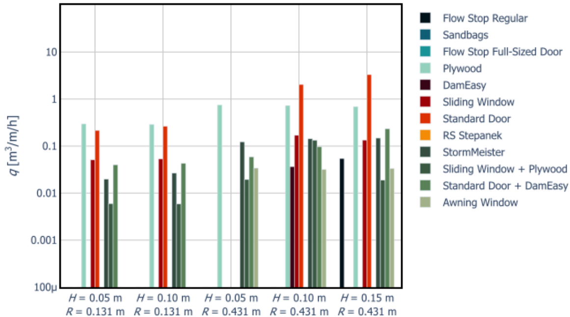
Figure 52. Average leakage rate per unit width for the wave experiments in Phase 2 (MWB only). The figure does not include tests from the IT as no waves were run in that facility.
