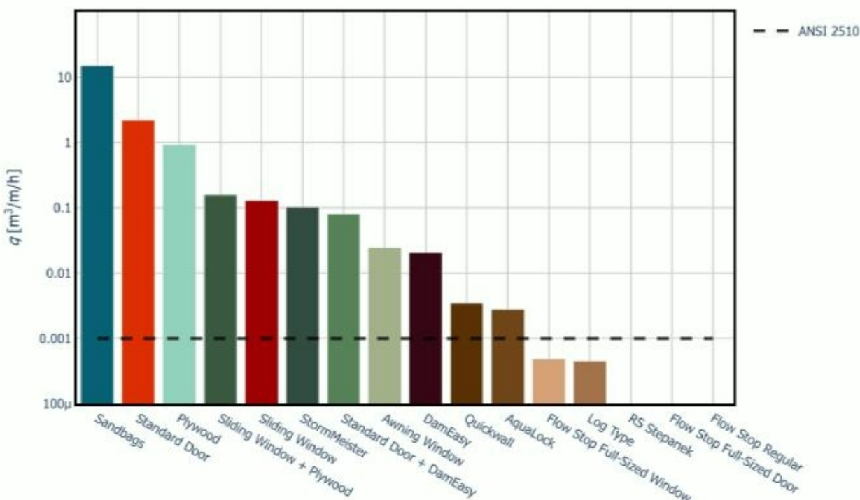
Figure 2. Summary of opening barrier performance in Phase 2 experiments at water level (0.585 m). Leakage rates are presented as volume flows per unit meter, and the ANSI 2510 threshold for opening barriers is represented by a dashed black line.
