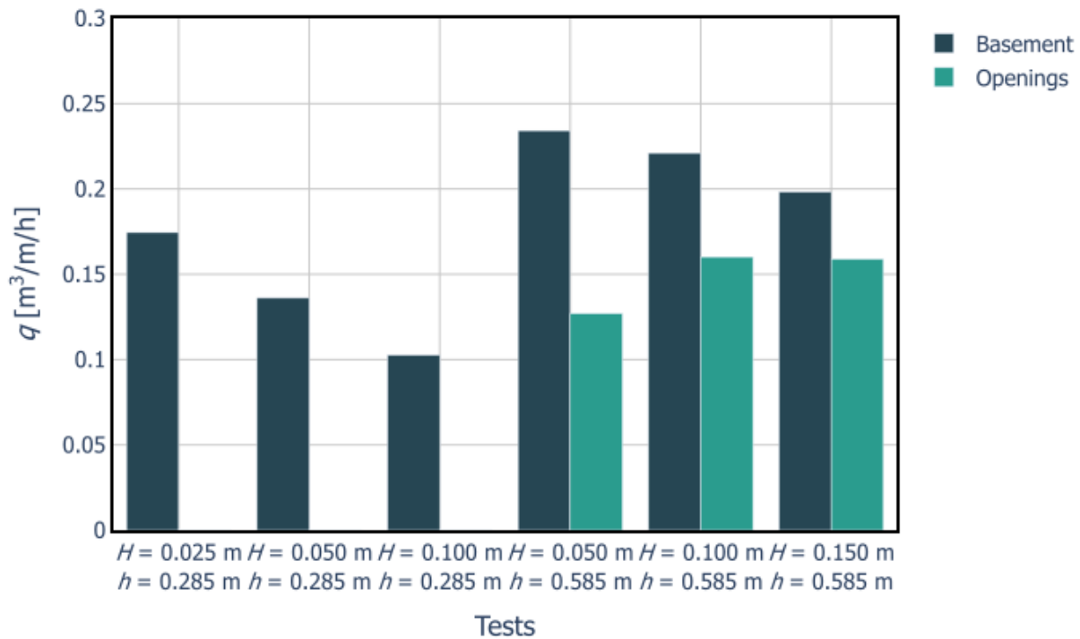
Figure 41. Leakage rates per unit length for Phase 1 superstructure under the influence of various combinations of water depth and zero-moment spectral wave height.
