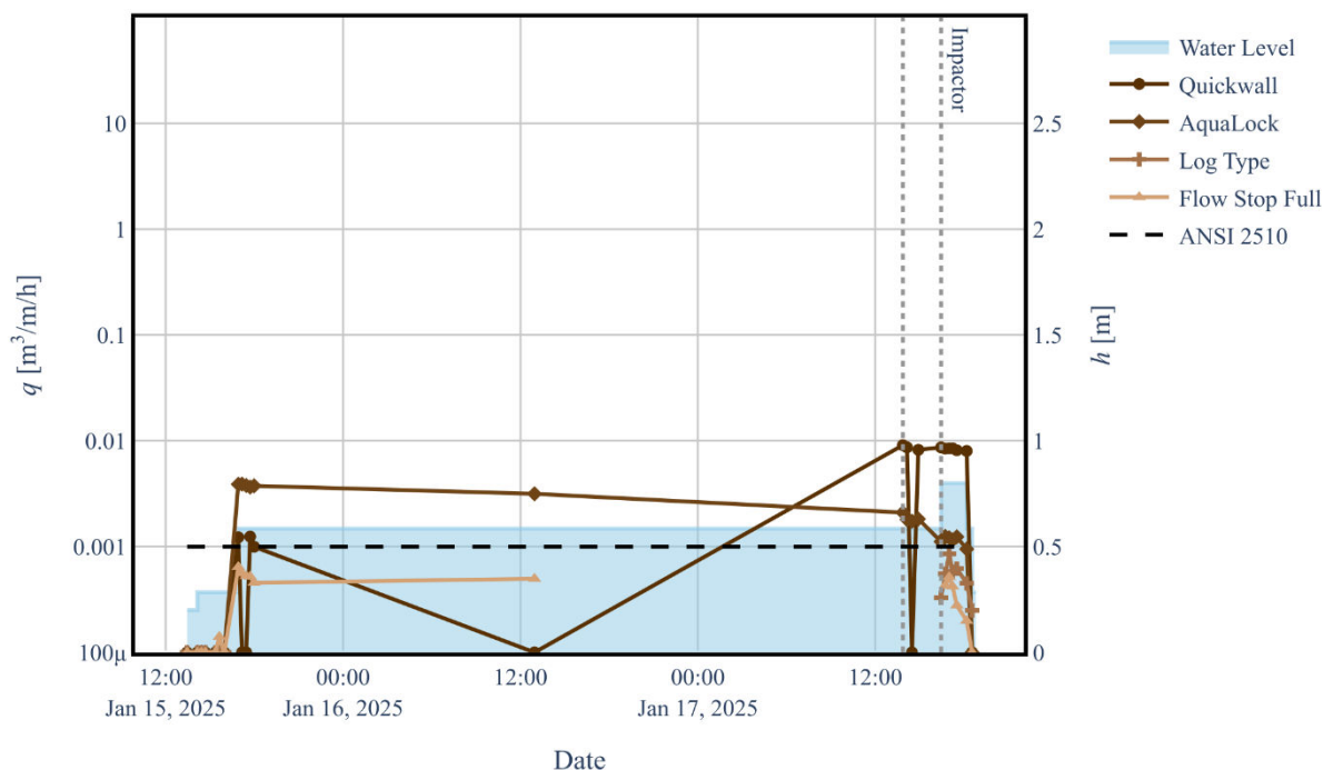
Figure 50. Leakage rate per unit width of the opening for the IT experiments.
