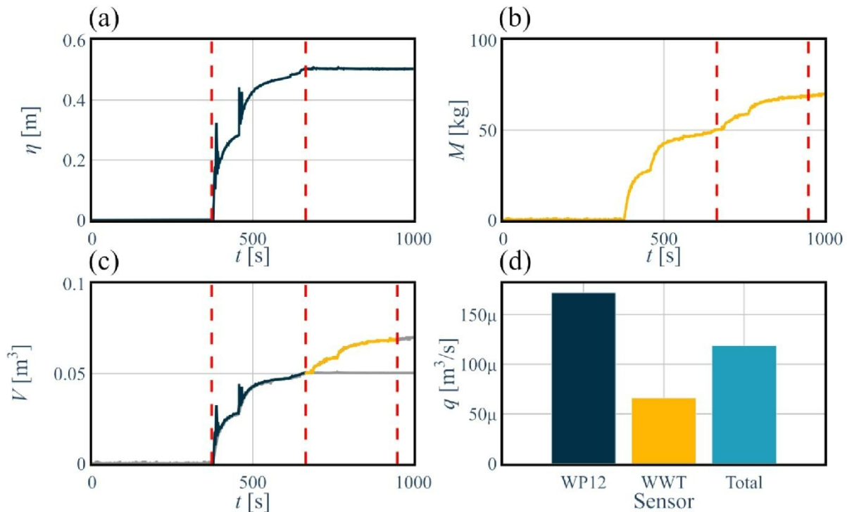
Figure 26. Measurement of overtopping rates. Example taken from Phase 2: TSE – Flow stop regular cushion on the west door opening. (a) water level measurements (WP12) in small tank; (b) weight tank measurements (WWT); (c) combined volume measurements from the two measurement methods; and (d) average overtopping rates measurements from two methods.
