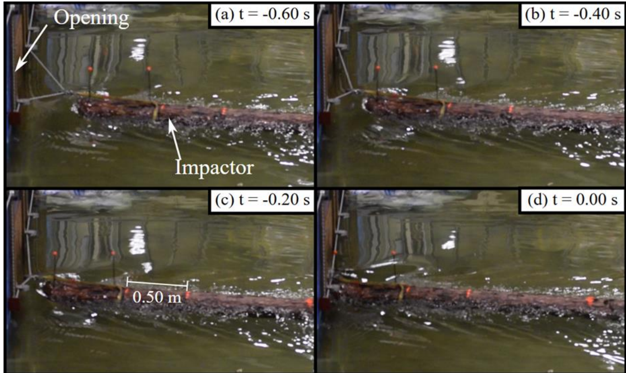
Figure 30. Debris impact testing in Phase 2 in the MWB showing the approach of the debris to a plywood barrier protecting a window opening. The time is provided in reference to the impact time.
