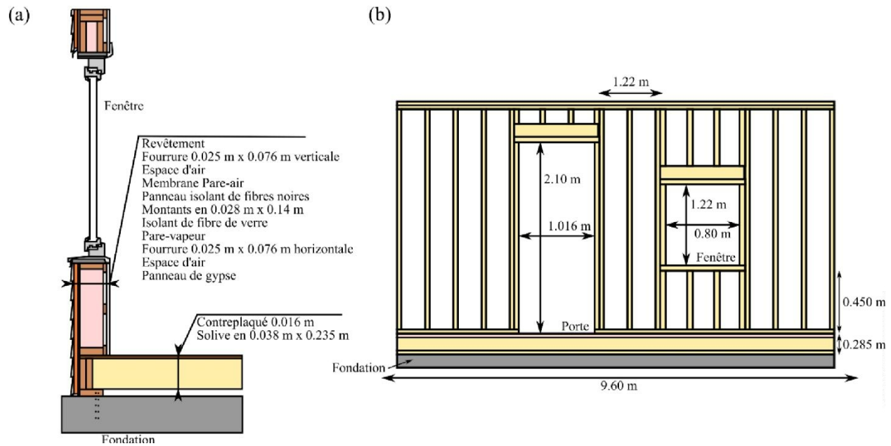
Figure 9. Phase 1 superstructure based on Ontario Building Code. (a) Cross-section of the superstructure; (b) front view of the superstructure.
